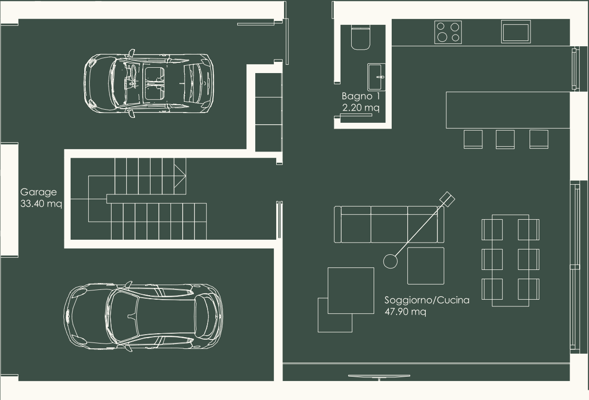
Piano terreno
