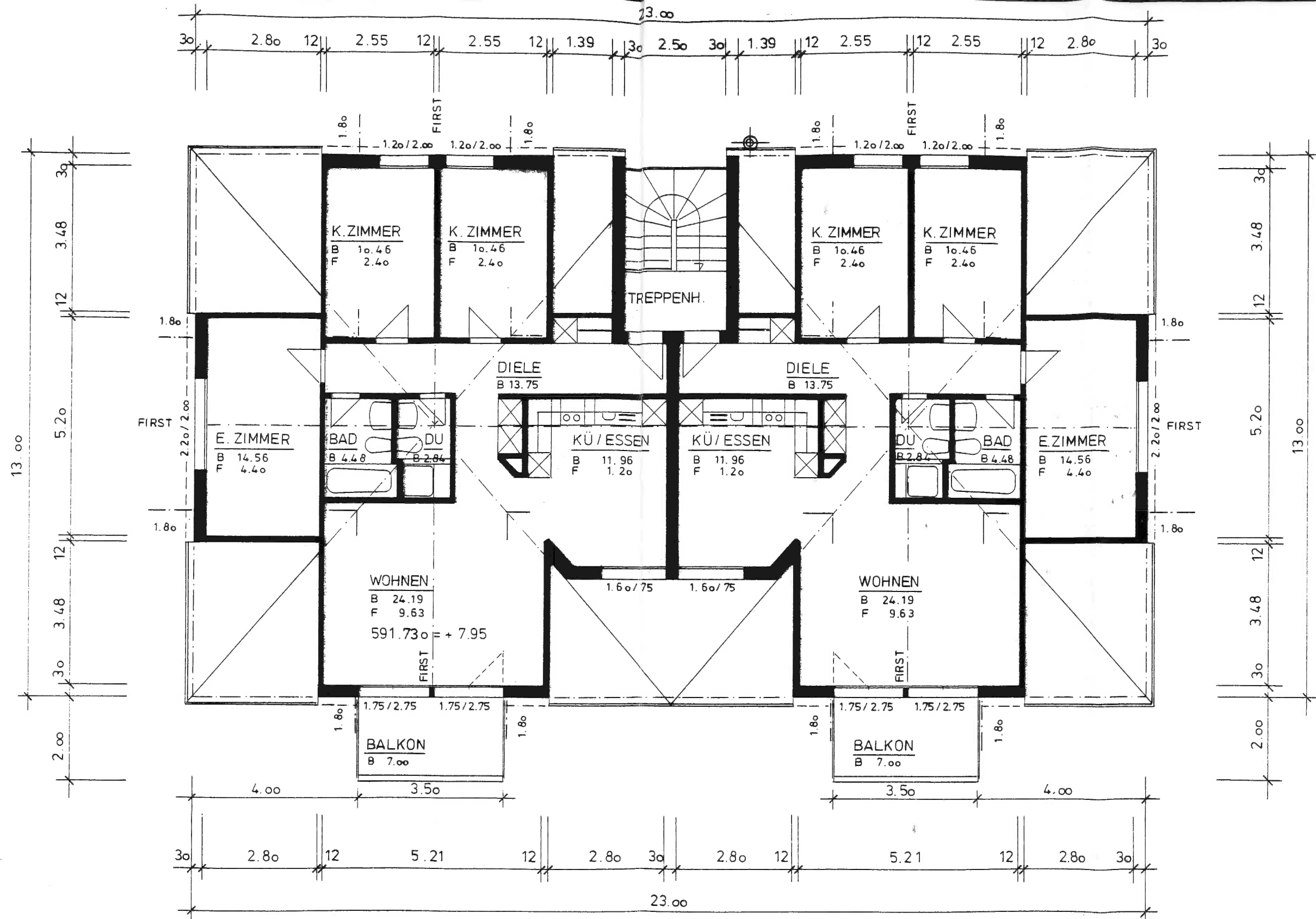
GRUNDRISS 2DG
