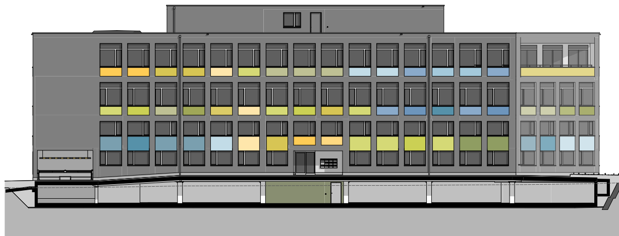
Fassade Northwest
