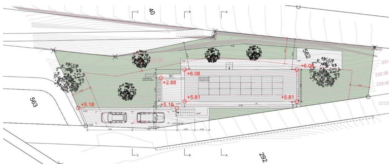
PIANO MODINE 1:100
