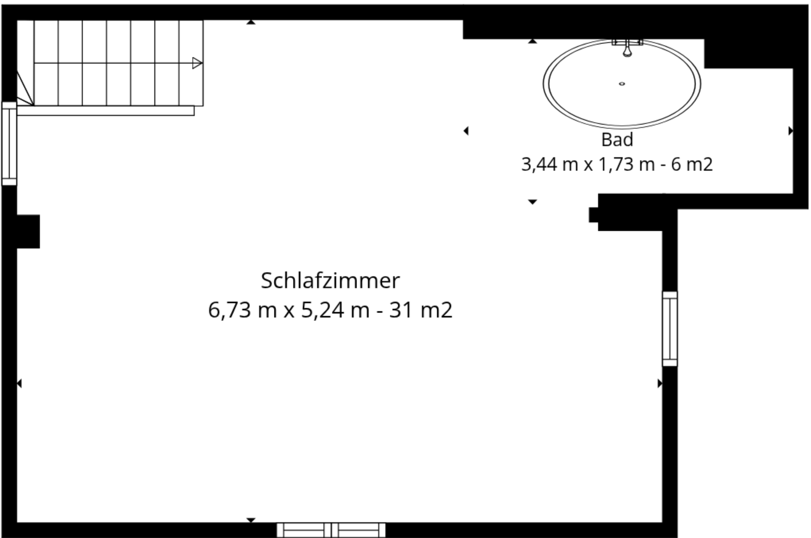
2. Stock
