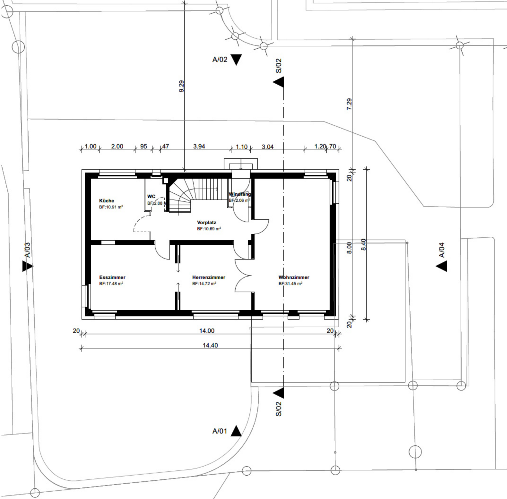
GURNDRISS EG
