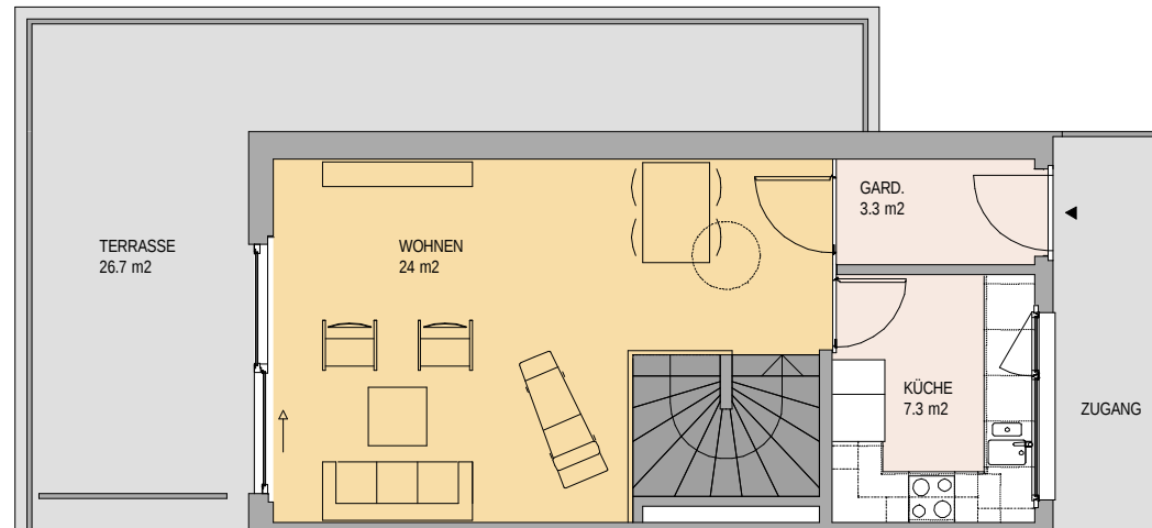
GRUNDRISS ATTIKA
